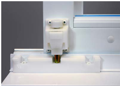
Three-position kick lock (550, Element)
